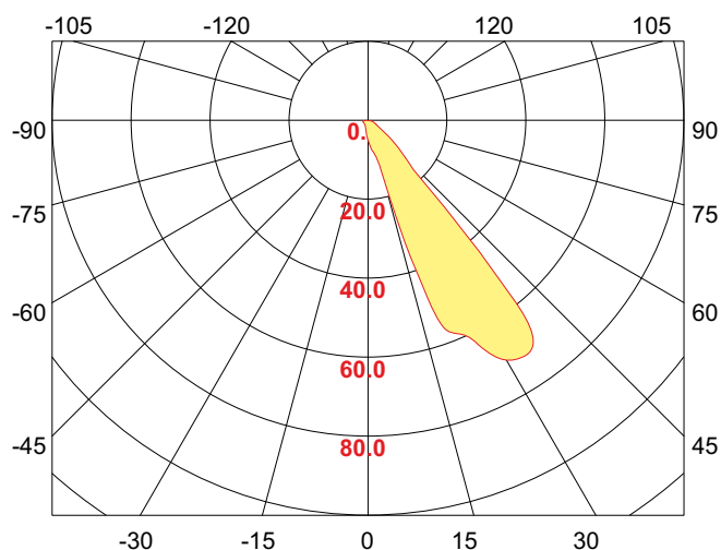
Intensity(unit:cd) C0-180
