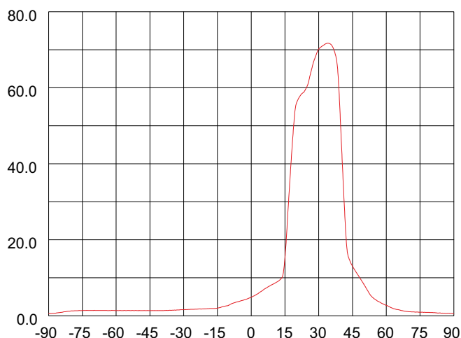
Intensity(unit:cd)C0-180 av(50%)=23.5 \theta
